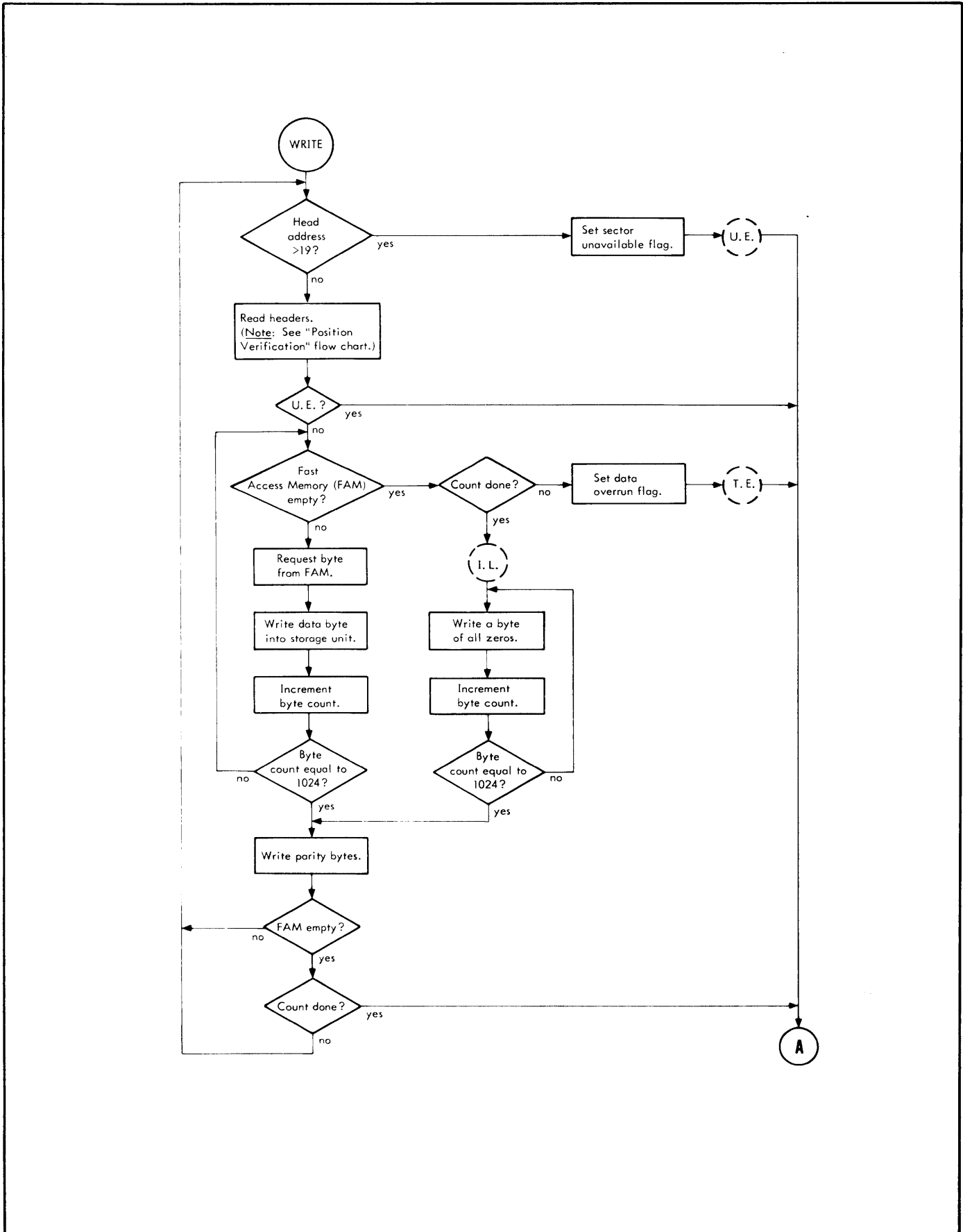
Figure 12. Write Order
