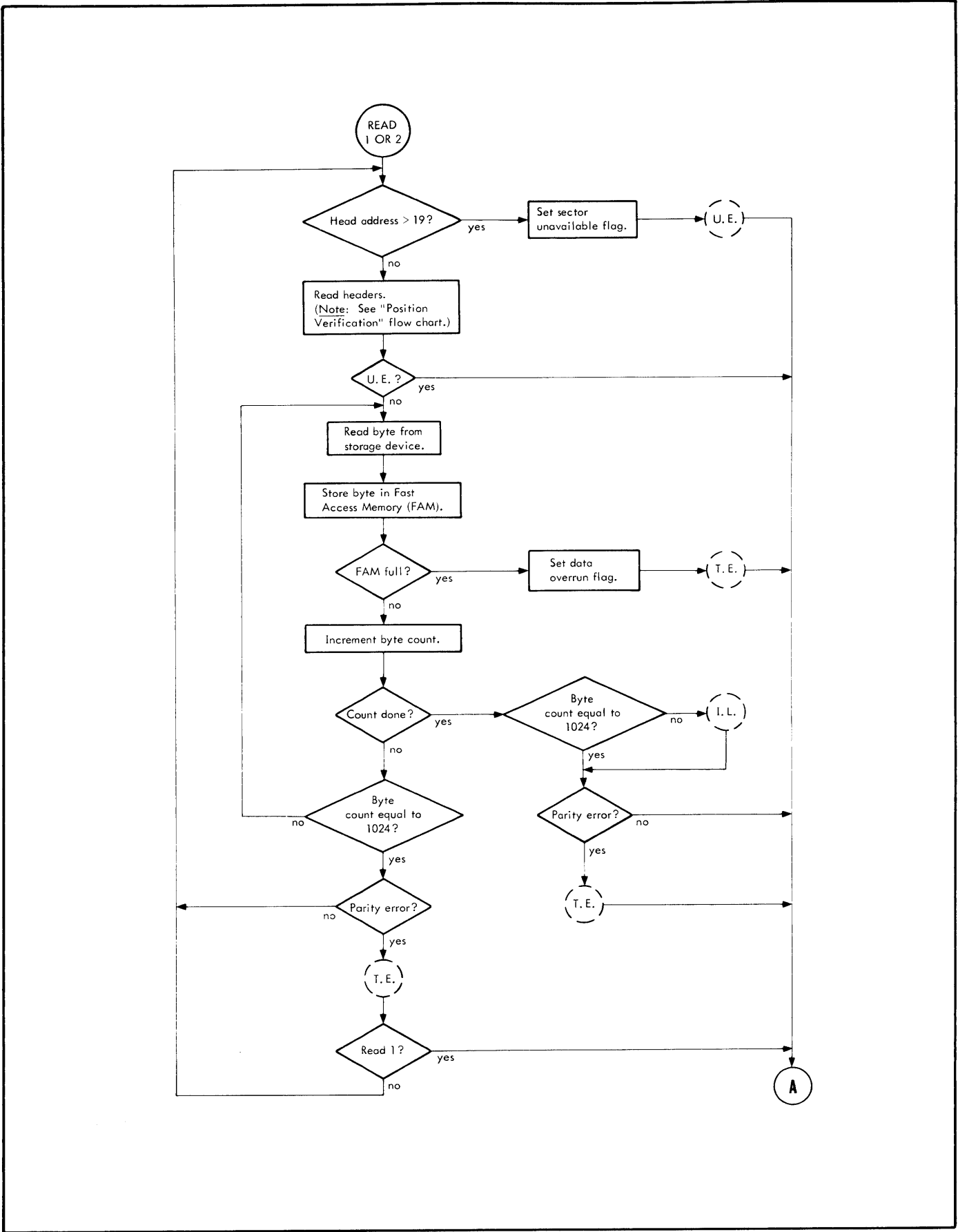
Figure 14. Read Orders
